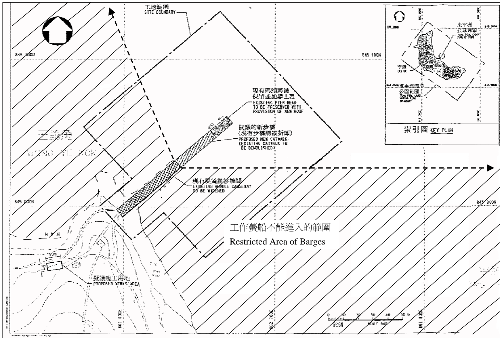
Figure 3: Improvement Works to Tung Ping Chau Public Pier – Restricted Area of Barges
