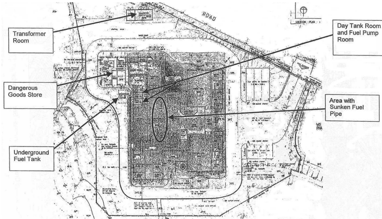
Figure 2 Provision of Cremators at Wo Hop Shek Crematorium (和合石火葬場重置火化爐工程)
