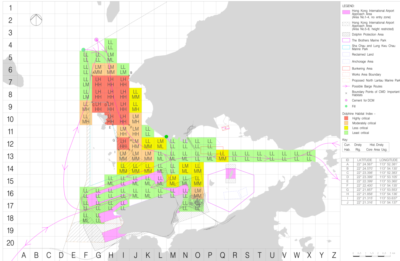
Figure 7-5b: Dolphin Habitat Index and Marine Travel Routes After I-2RS and Before Designation of NLMP
