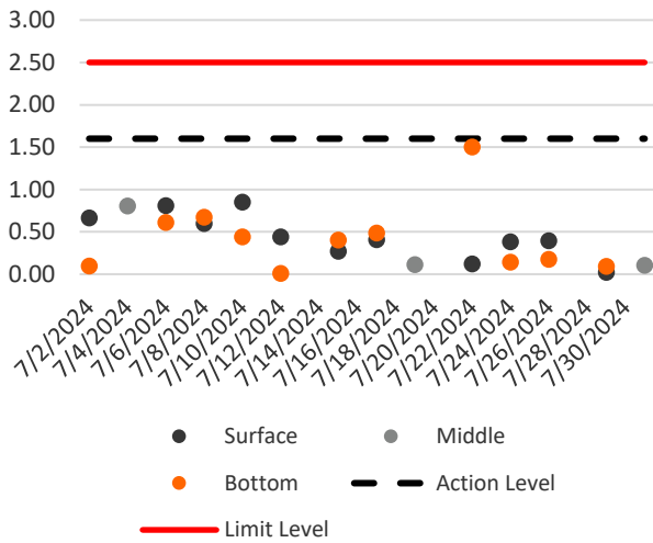
Turbidity (Depth-Averaged) during Mid-Ebb
