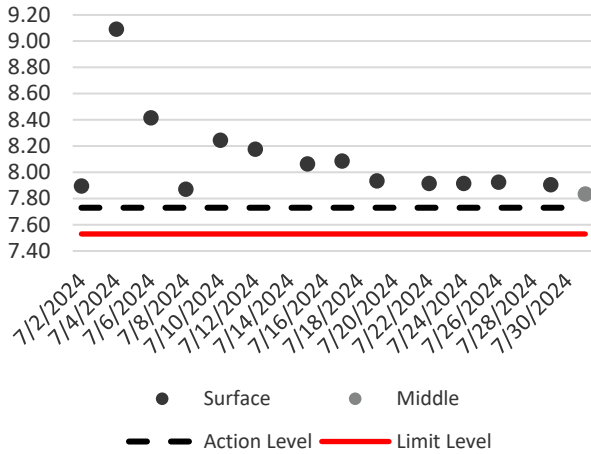
Dissolved Oxygen (Surface & Middle) during Mid-Ebb
