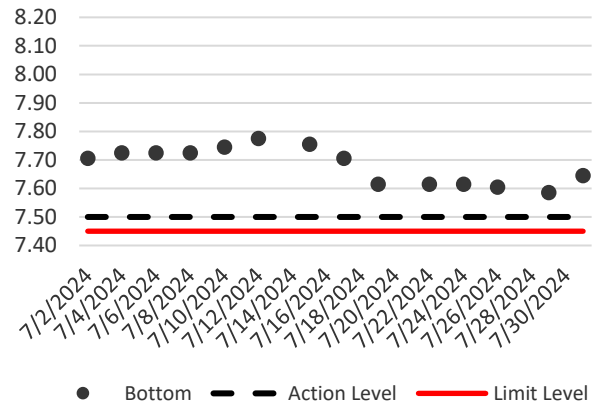
Dissolved Oxygen (Bottom) during Mid-Ebb
