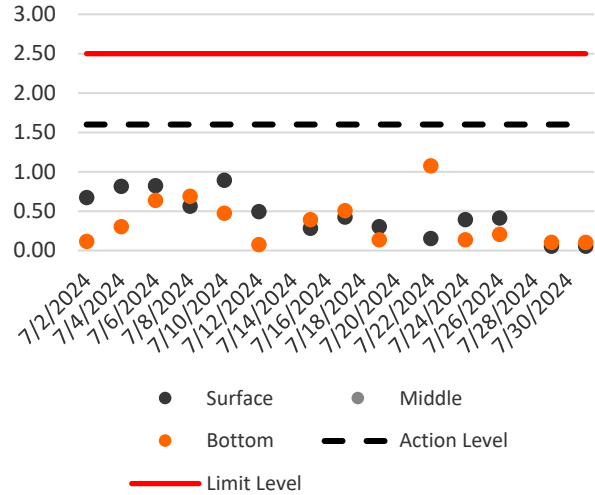
Turbidity (Depth-Averaged) during Mid-Flood
