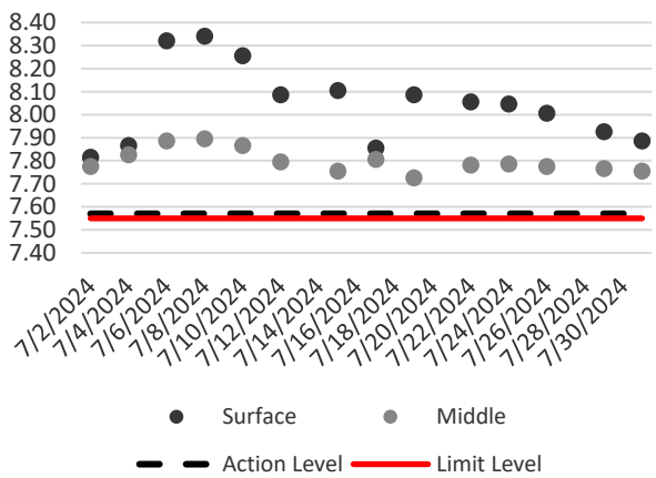
Dissolved Oxygen (Surface & Middle) during Mid-Flood
