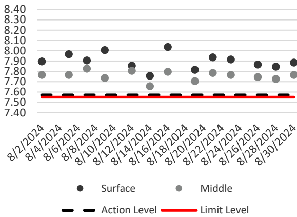
Dissolved Oxygen (Surface & Middle) during Mid-Ebb
