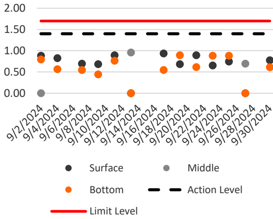
Turbidity (Depth-Averaged) during Mid-Ebb
