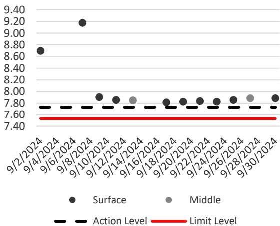
Dissolved Oxygen (Surface & Middle) during Mid-Flood
