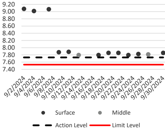
Dissolved Oxygen (Surface & Middle) during Mid-Ebb
