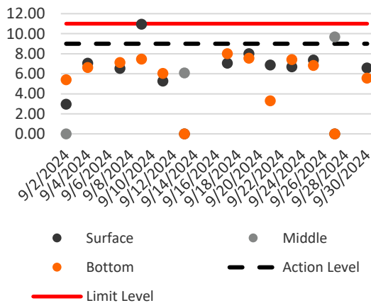
Suspended Solids (Depth Average) during Mid-Ebb
