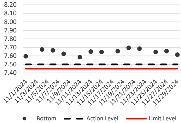
Dissolved Oxygen (Bottom) during Mid-Ebb
