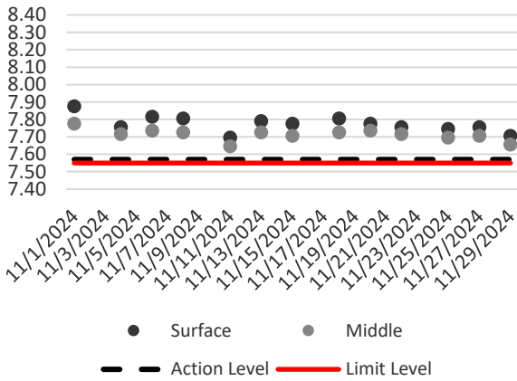
Dissolved Oxygen (Surface & Middle) during Mid-Ebb
