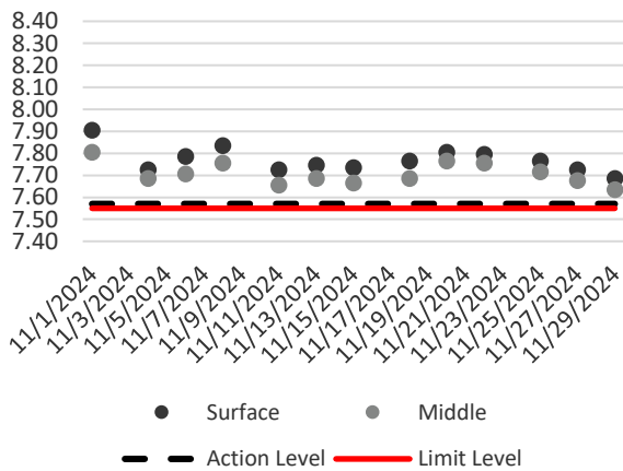
Dissolved Oxygen (Surface & Middle) during Mid-Flood
