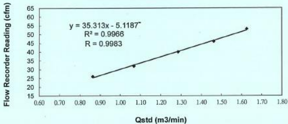
Sampler 1180 Calibration Curve Site: Tuen Mun (TM-RA2)
