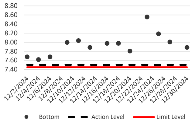
Dissolved Oxygen (Bottom) during Mid-Ebb
