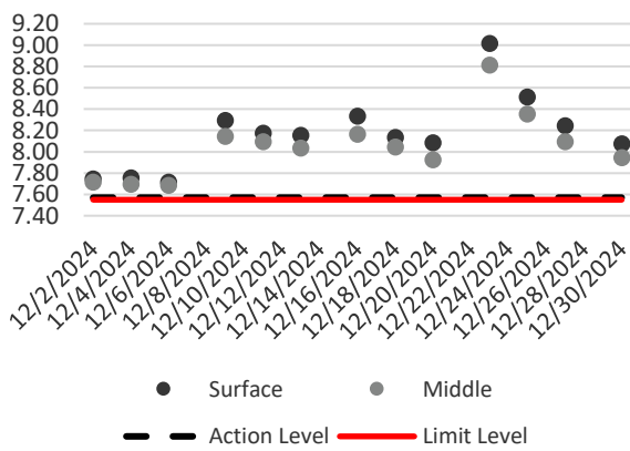
Dissolved Oxygen (Surface & Middle) during Mid-Flood
