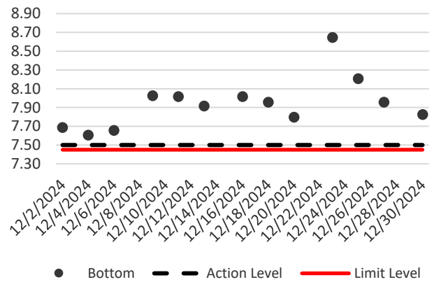
Dissolved Oxygen (Bottom) during Mid-Flood
