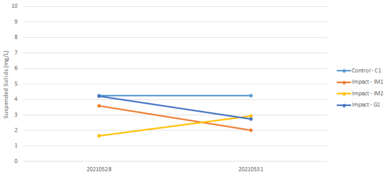
Suspended Solids (Depth-averaged) during Mid-Flood
