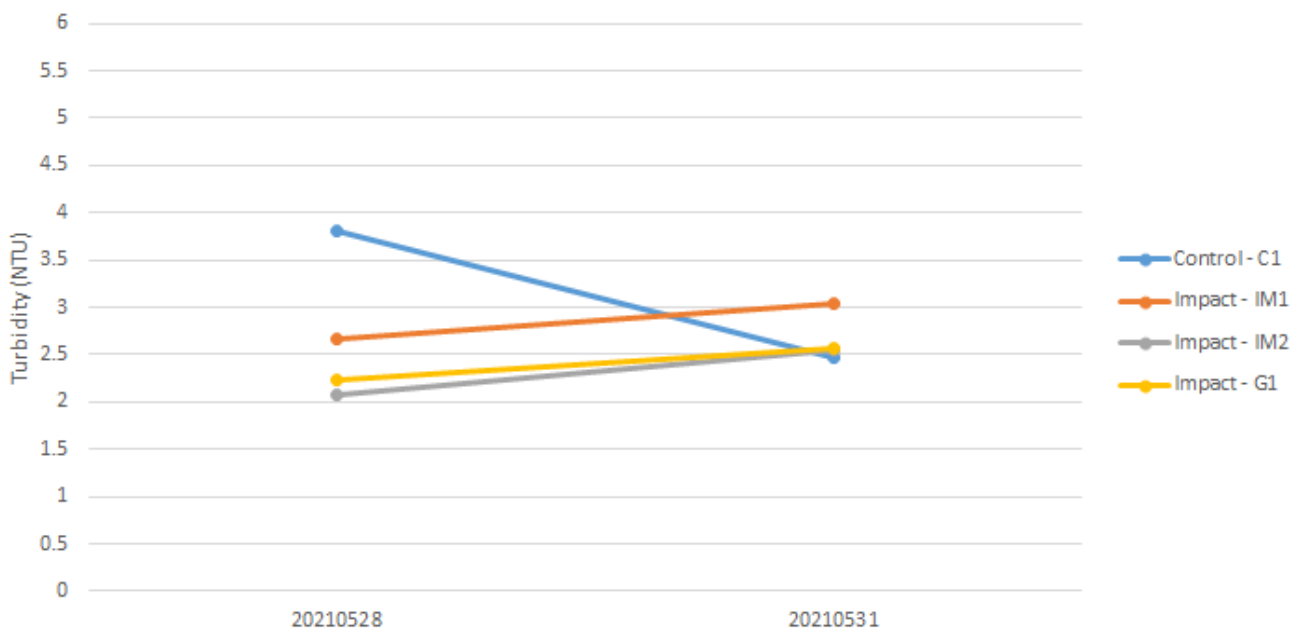
Turbidity (Depth-averaged) during Mid-Flood
