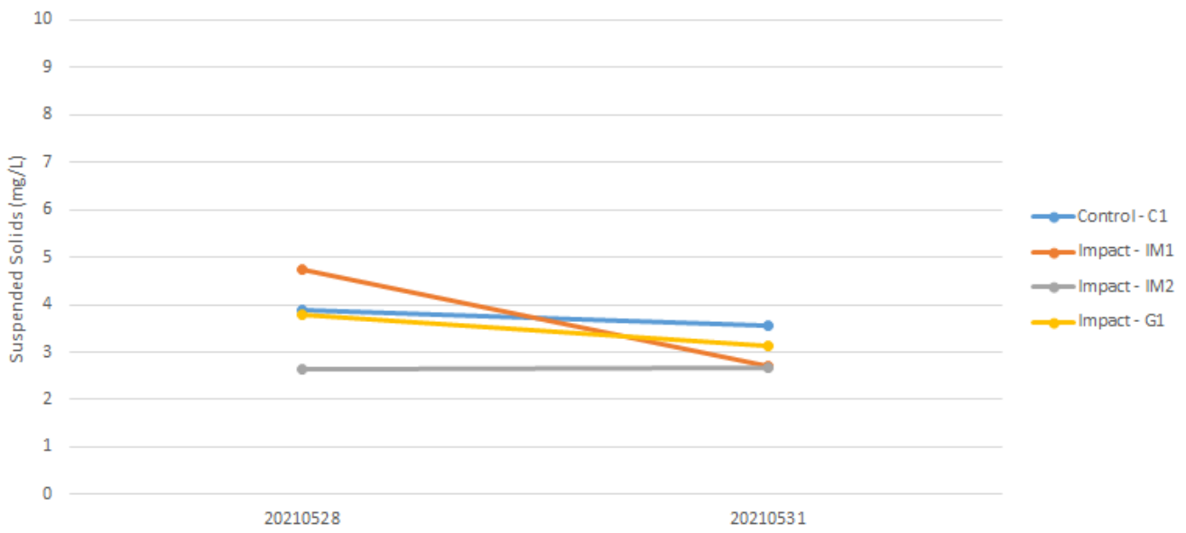
Suspended Solids (Depth-averaged) during Mid-Ebb
