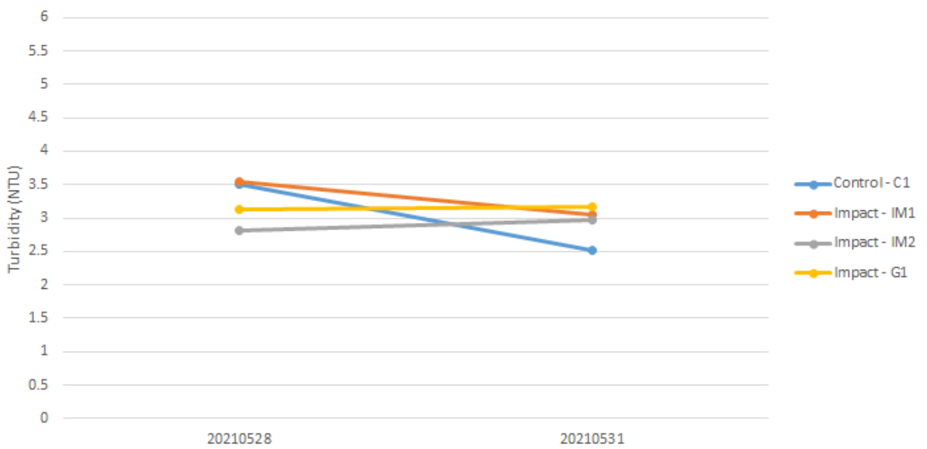
Turbidity (Depth-averaged) during Mid-Ebb
