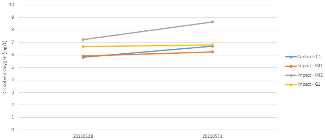
Dissolved Oxygen (Surface and Middle) during Mid-Ebb
