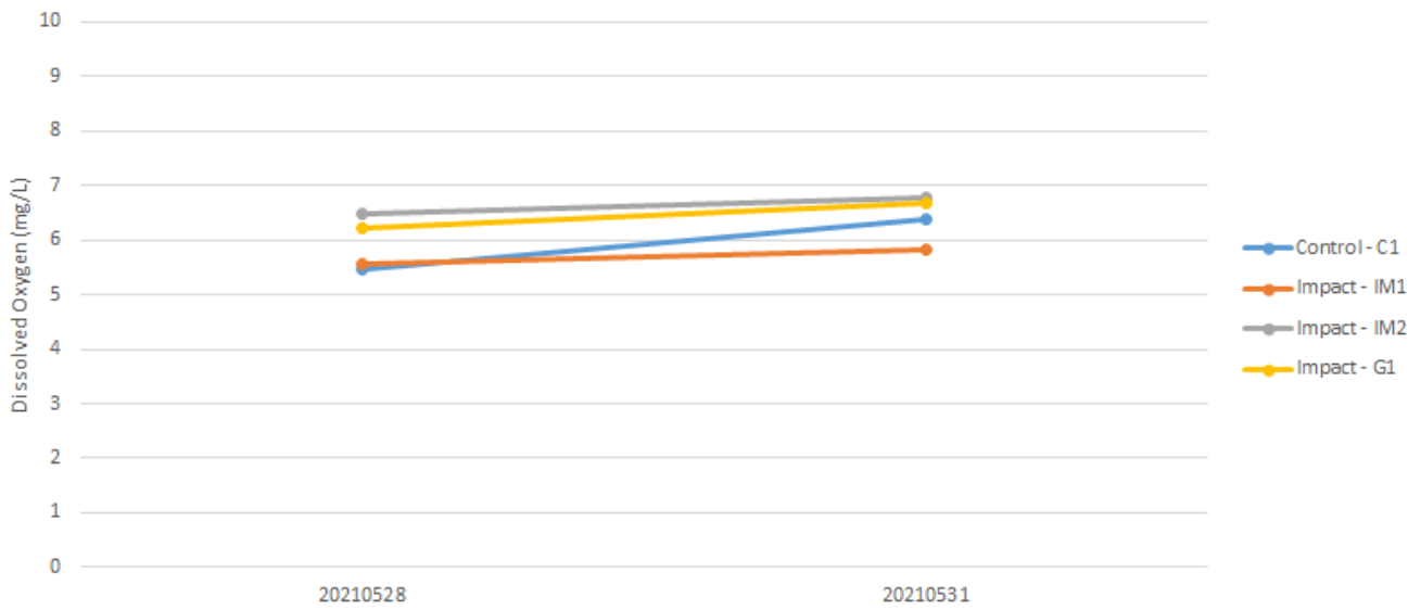
Dissolved Oxygen (Surface and Middle) during Mid-Flood
