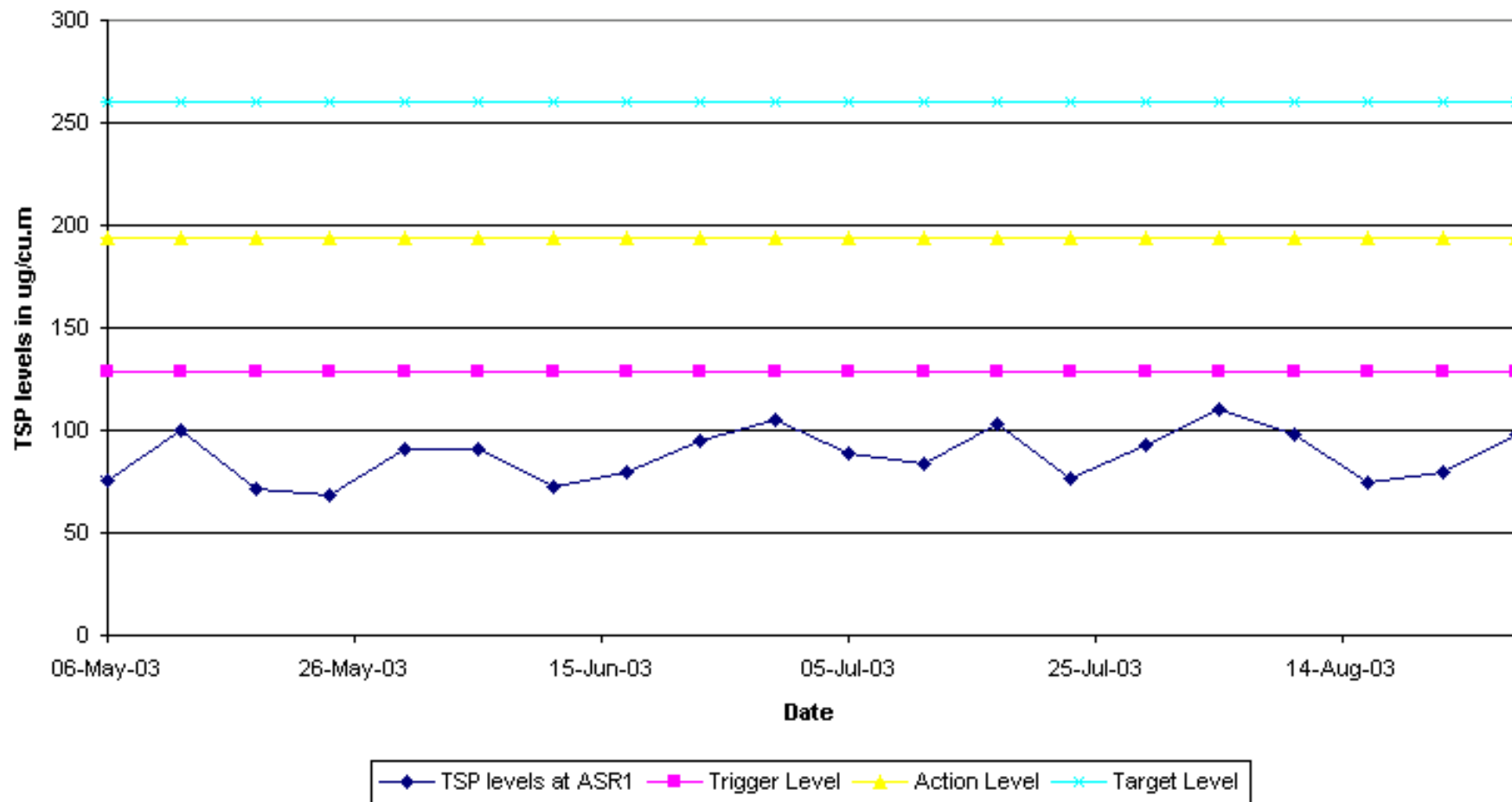
Figure 6.1 - Graphical Plot of 24-hour TSP Levels
