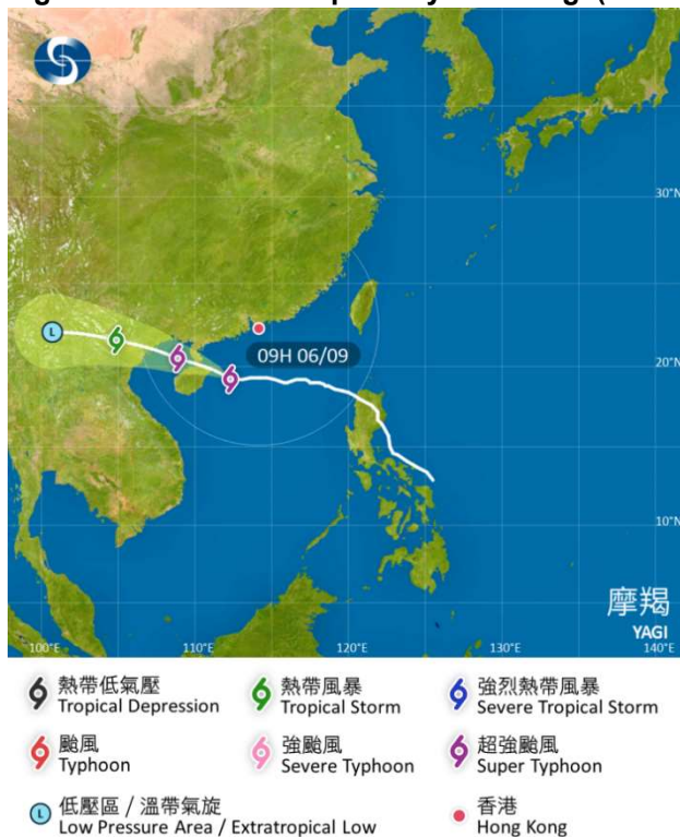
Figure 2.4: Track of Tropical Cyclone Yagi (Source: Hong Kong Observatory)
