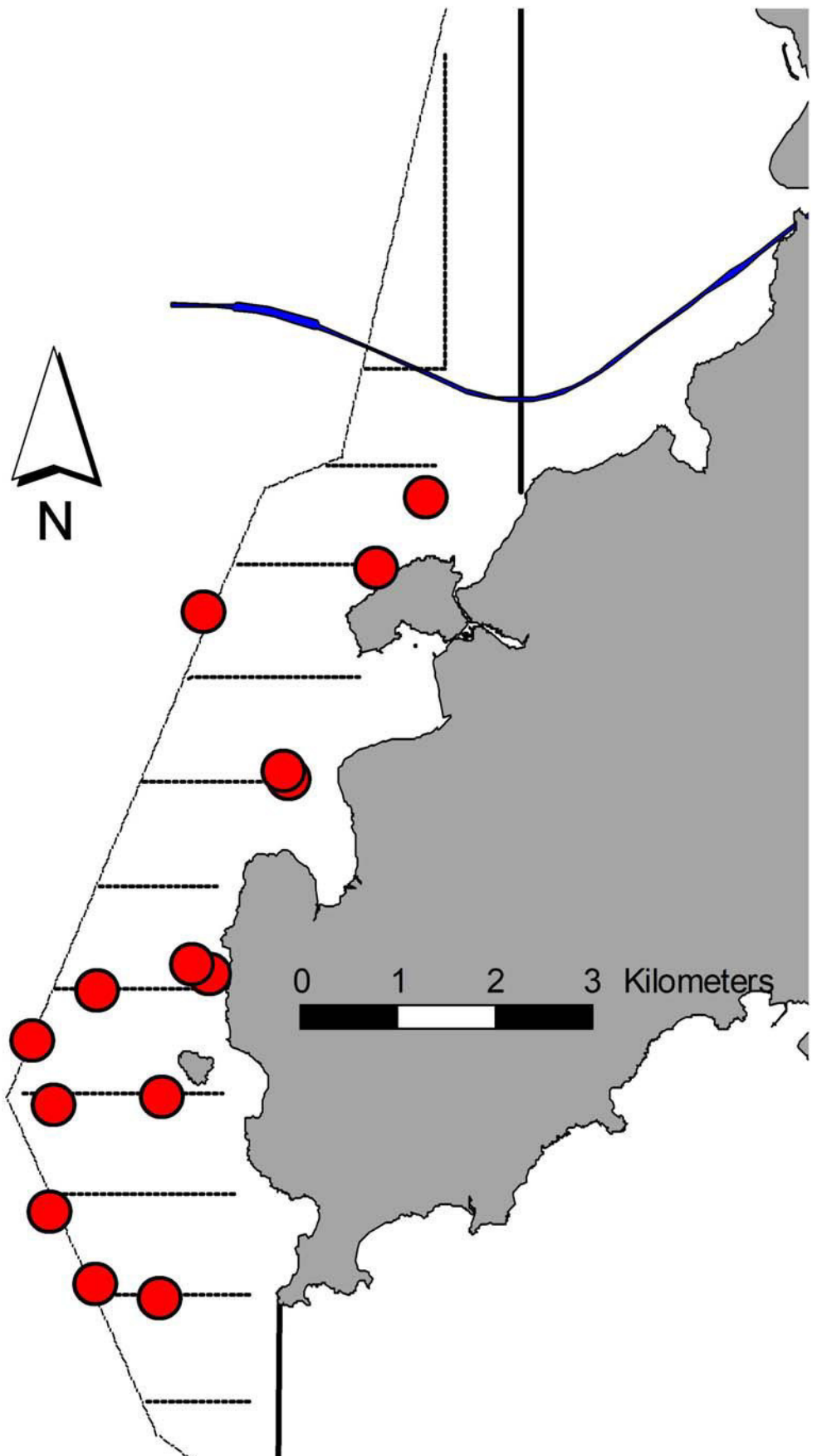
Figure 4. Distribution of Chinese White Dolphin Sighting during September 2018 HKLR09 Monitoring Surveys
