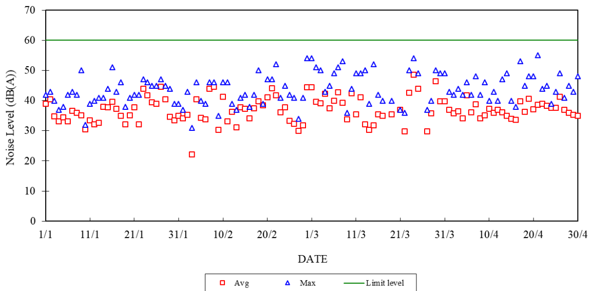
Construction Noise Monitoring in January 2024 - April 2024 NSR at School within Tai Wan San Tsuen 07:00-23:00 hrs on Holidays and 19:00-23:00 hrs on All Other Days
