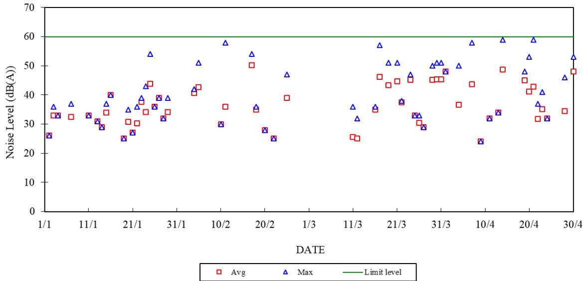
Construction Noise Monitoring in January 2024 - April 2024 NSR at Long Tsai Tsuen/Hung Shing Ye 07:00-23:00 hrs on Holidays and 19:00-23:00 hrs on All Other Days
