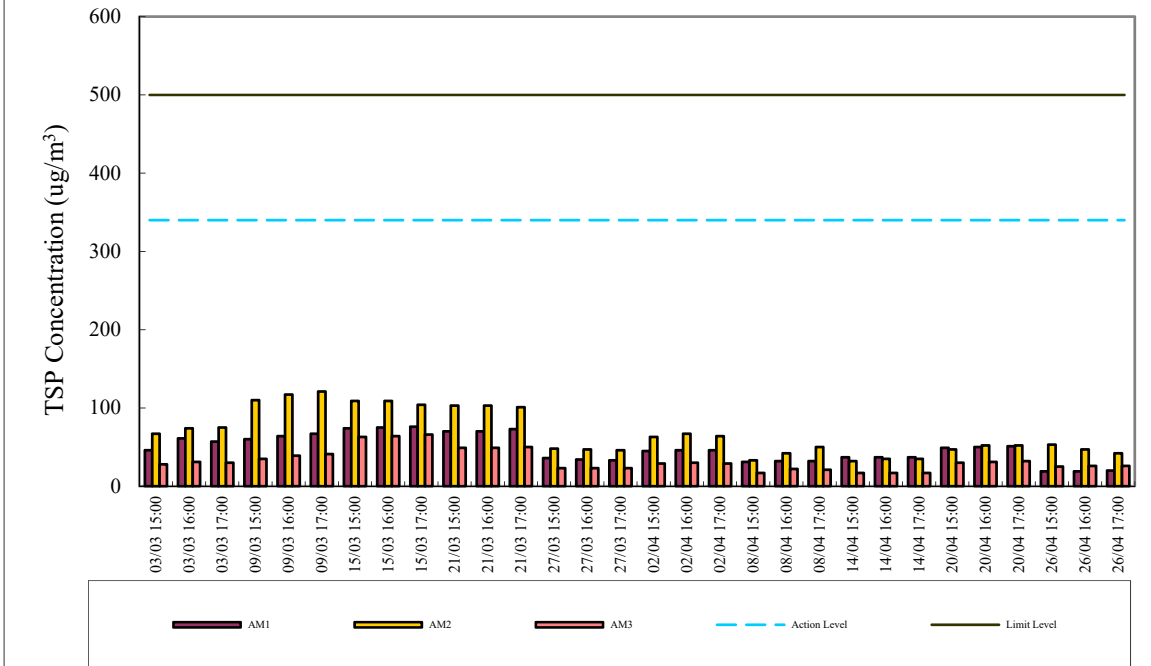
1-hr TSP Air Monitoring Data (March 2024 - April 2024)
