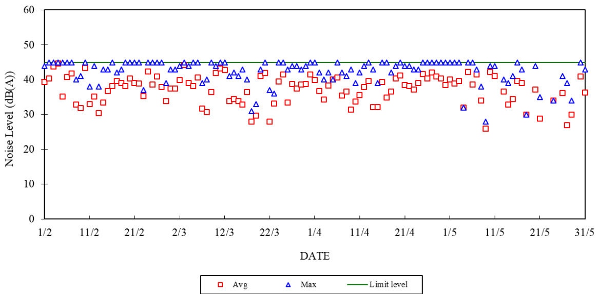
Construction Noise Monitoring in February 2024 - May 2024 NSR at School within Tai Wan San Tsuen 23:00-07:00 hrs of Next Day
