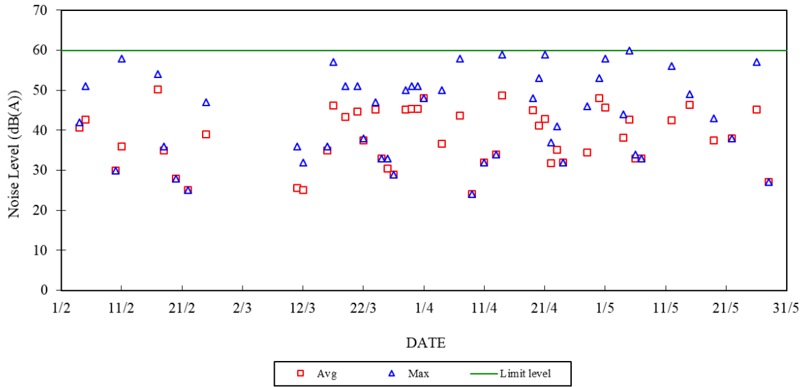
Construction Noise Monitoring in February 2024 - May 2024 NSR at Long Tsai Tsuen/Hung Shing Ye 07:00-23:00 hrs on Holidays and 19:00-23:00 hrs on All Other Days
