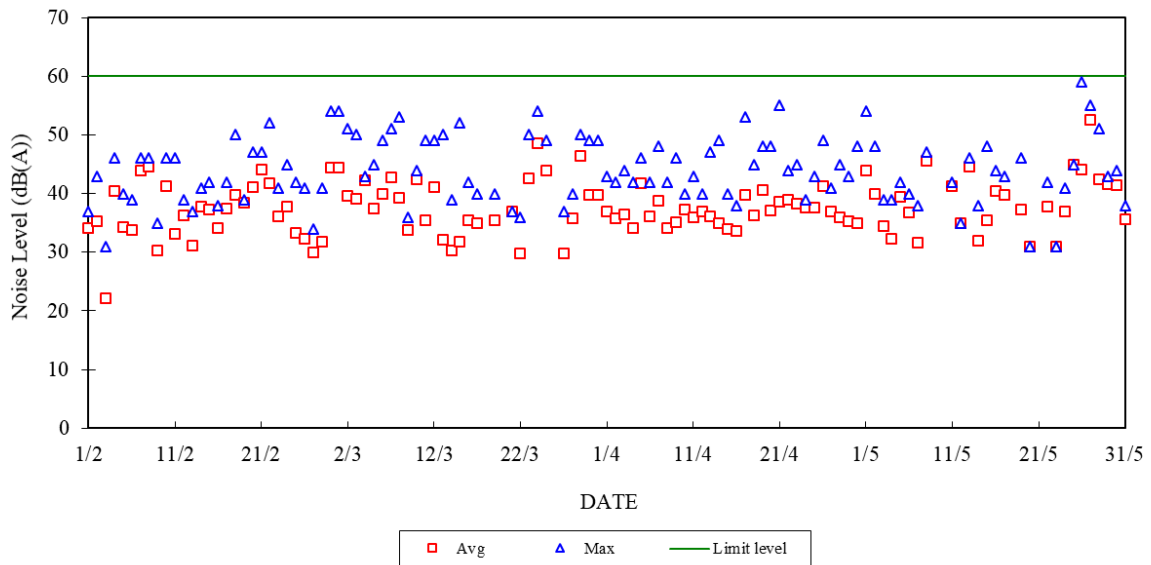
Construction Noise Monitoring in February 2024 - May 2024 NSR at School within Tai Wan San Tsuen 07:00-23:00 hrs on Holidays and 19:00-23:00 hrs on All Other Days
