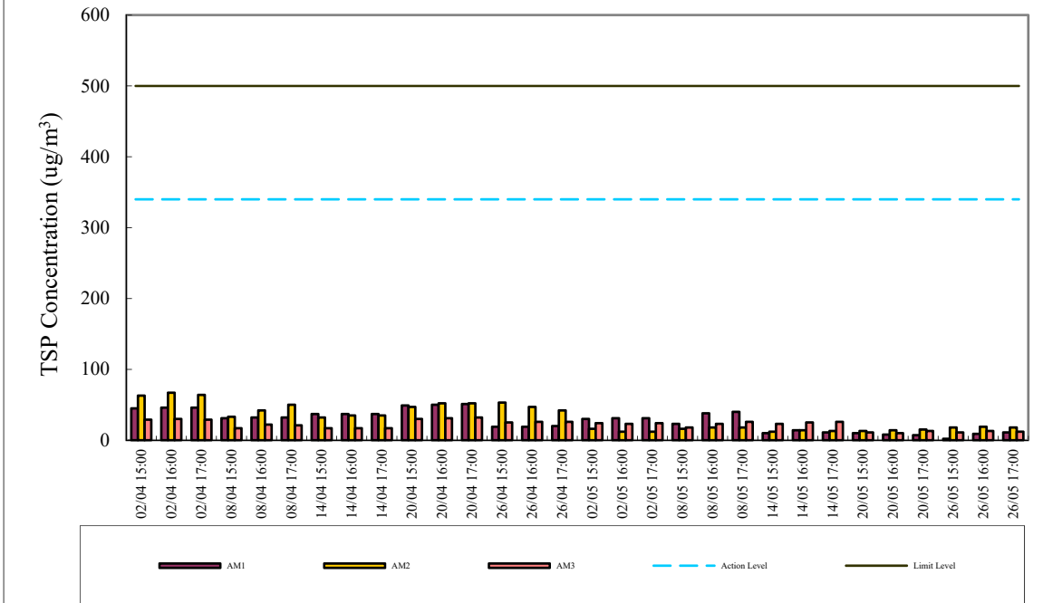
1-hr TSP Air Monitoring Data (April 2024 - May 2024)
