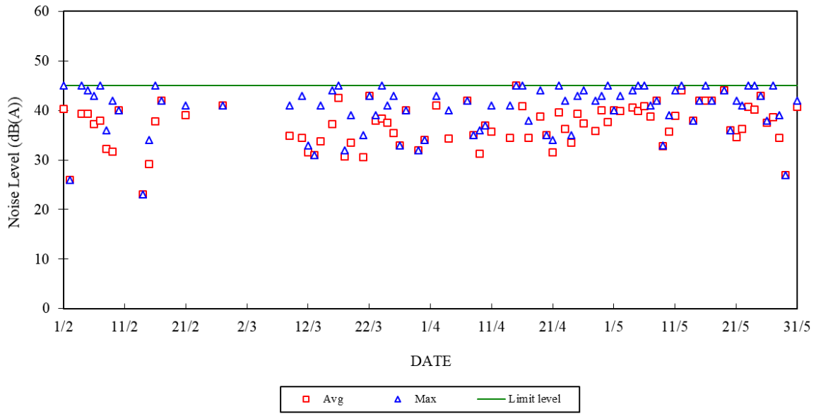
Construction Noise Monitoring in February 2024 - May 2024 NSR at Long Tsai Tsuen/Hung Shing Ye 23:00-07:00 hrs of Next Day
