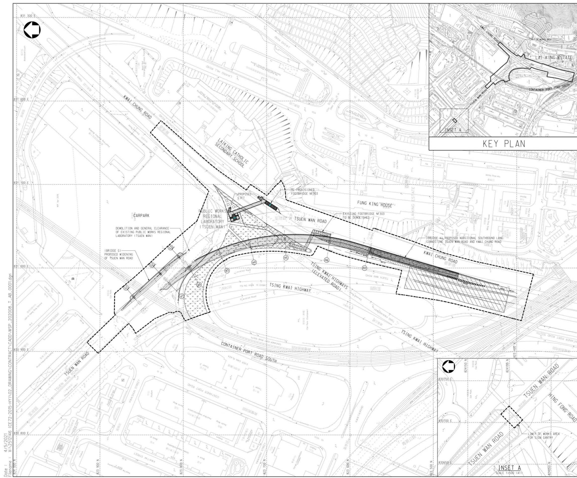
Figure 1.1 Project Layout
