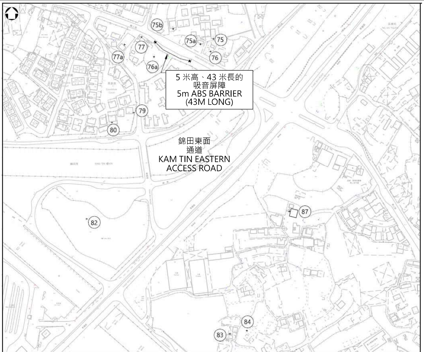
Figure 3 – Direct Road Traffic Noise Mitigation Measure For Kam Tin Eastern Access Road (South & West Section)
