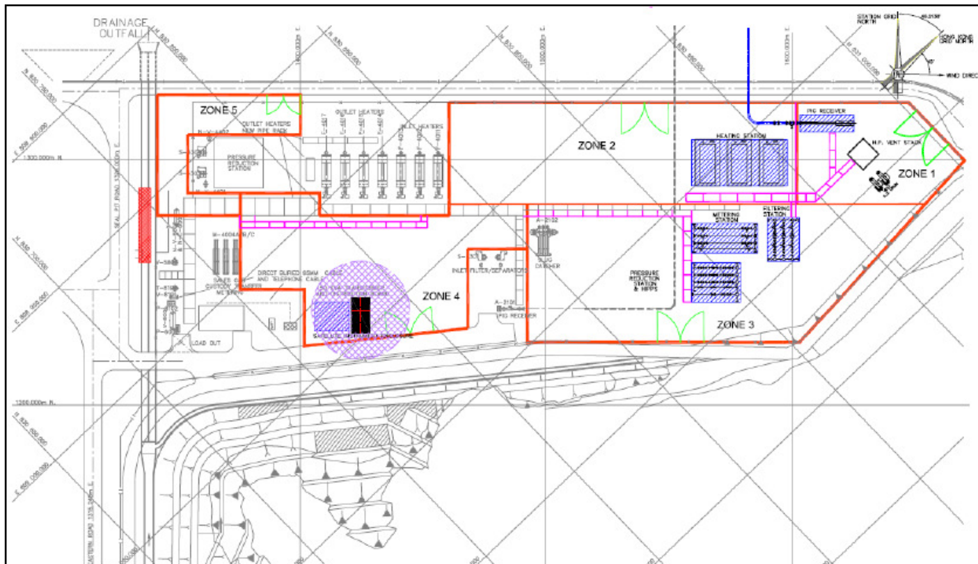
Construction of the co-located GRS at BPPS (Stage 4)
