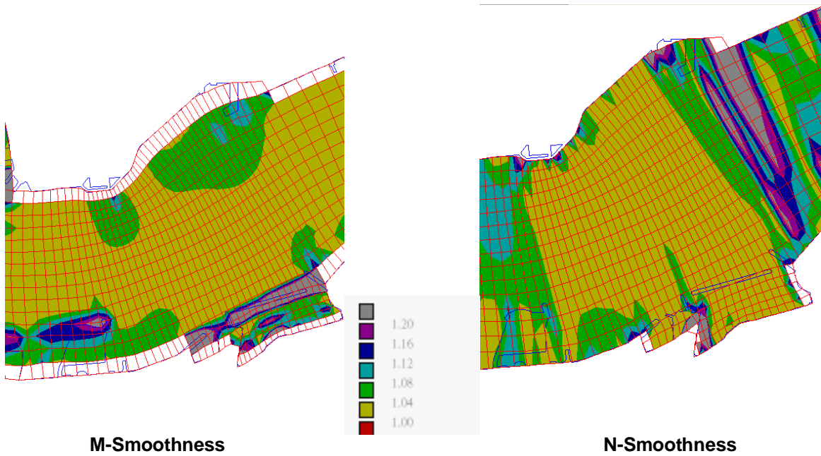
Figure C3 Grid Smoothness of VH Model
