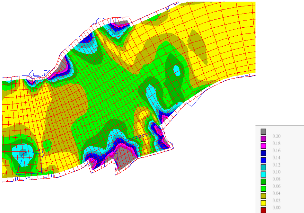
Figure C2 Grid Orthogonality of VH Model
