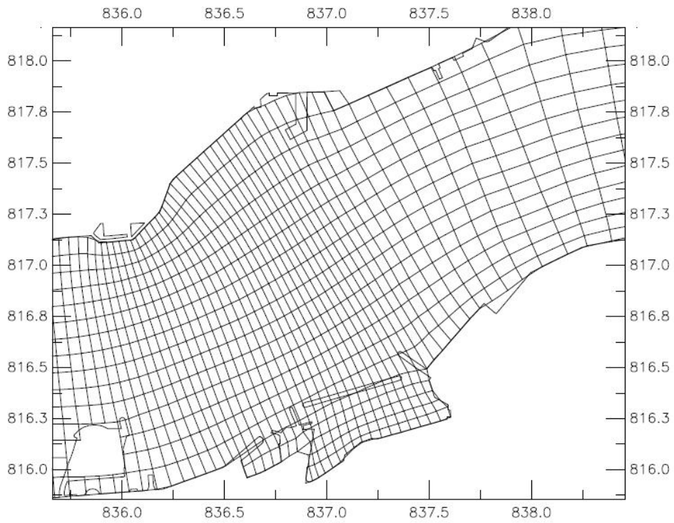
Figure C1b Grid Schematization of VH Model – Close Up at Hung Hom and Causeway Bay Typhoon Shelter
