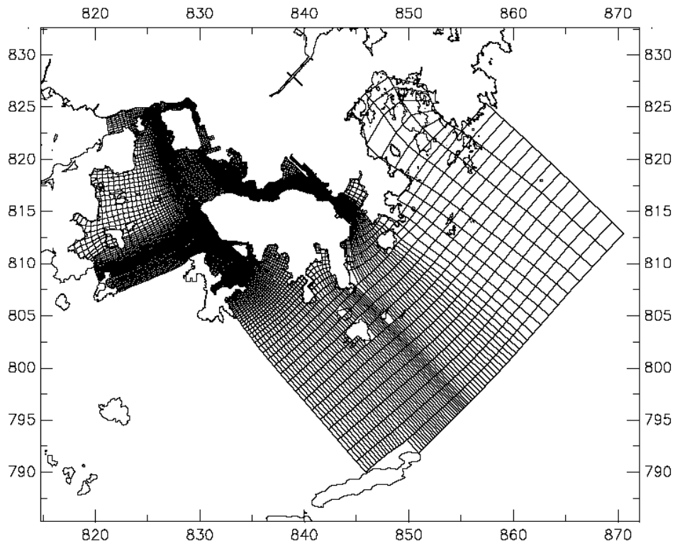
Figure C1a Coverage and Grid Schematization of VH Model – Overview
