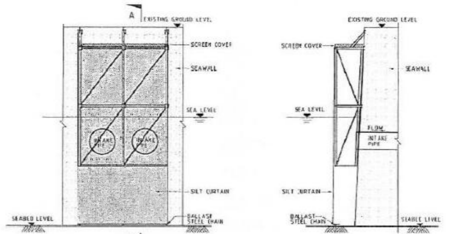
TYPICAL DETAILS FOR SILT SCREEN OVER INTAKE PIPES
