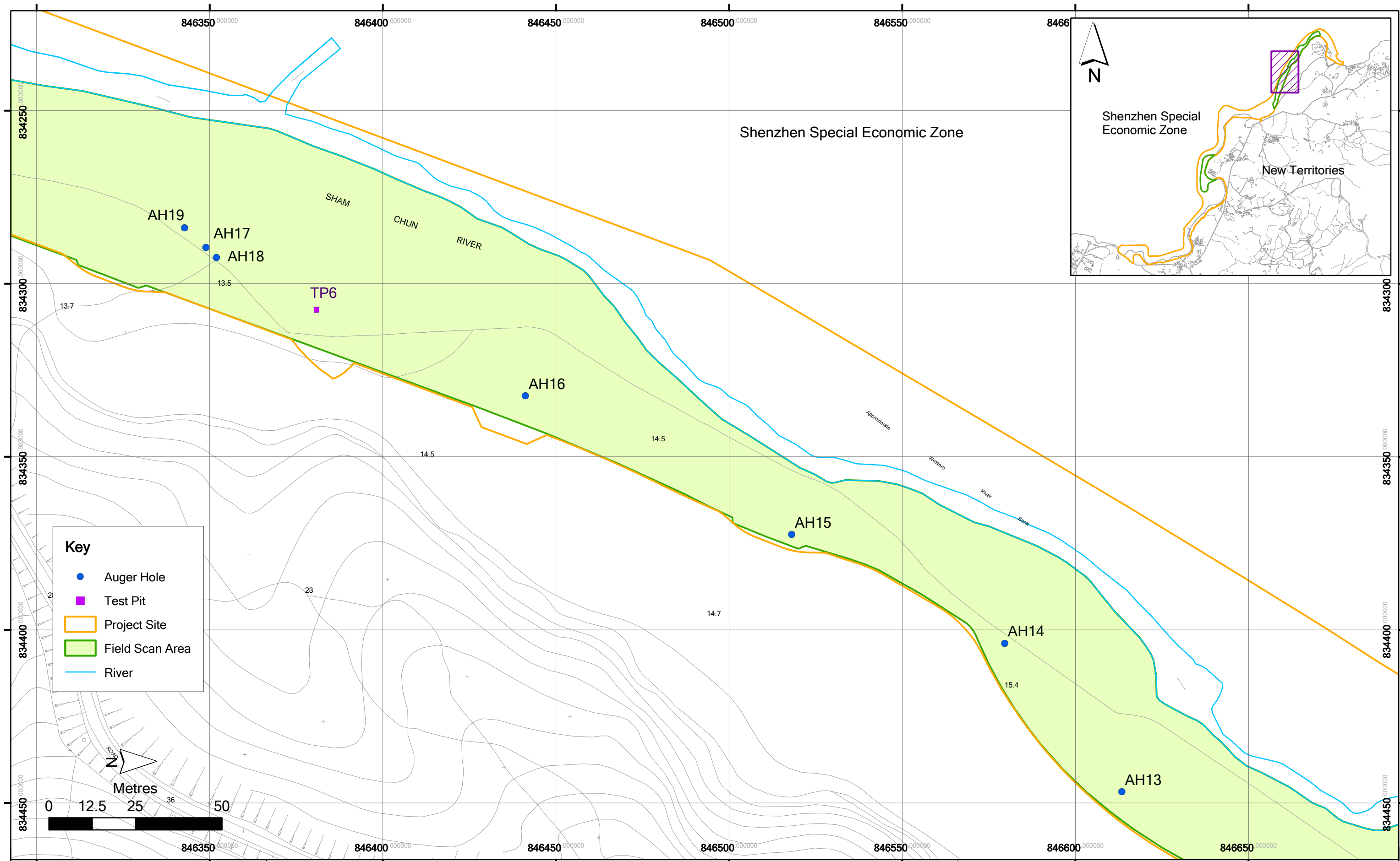
Figure 11.15 Layout Plan for Test Pits and Auger Holes Location and Topography of Pak Fu Shan Section
