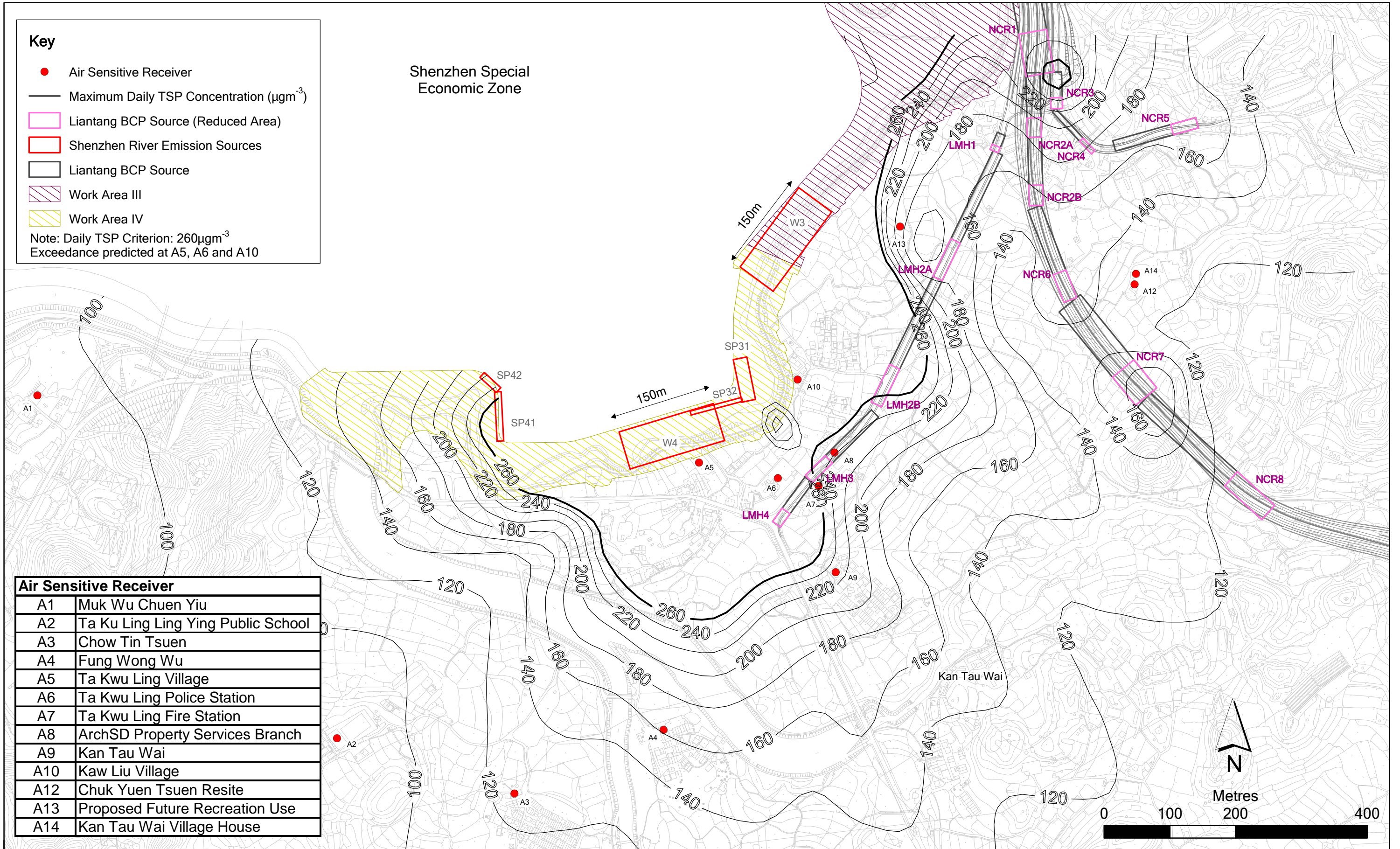
Figure 4.4 Unmitigated Maximum Daily TSP Concentration at 1.5m above ground (Scenario 1 - Active Works Areas Shift to South)
