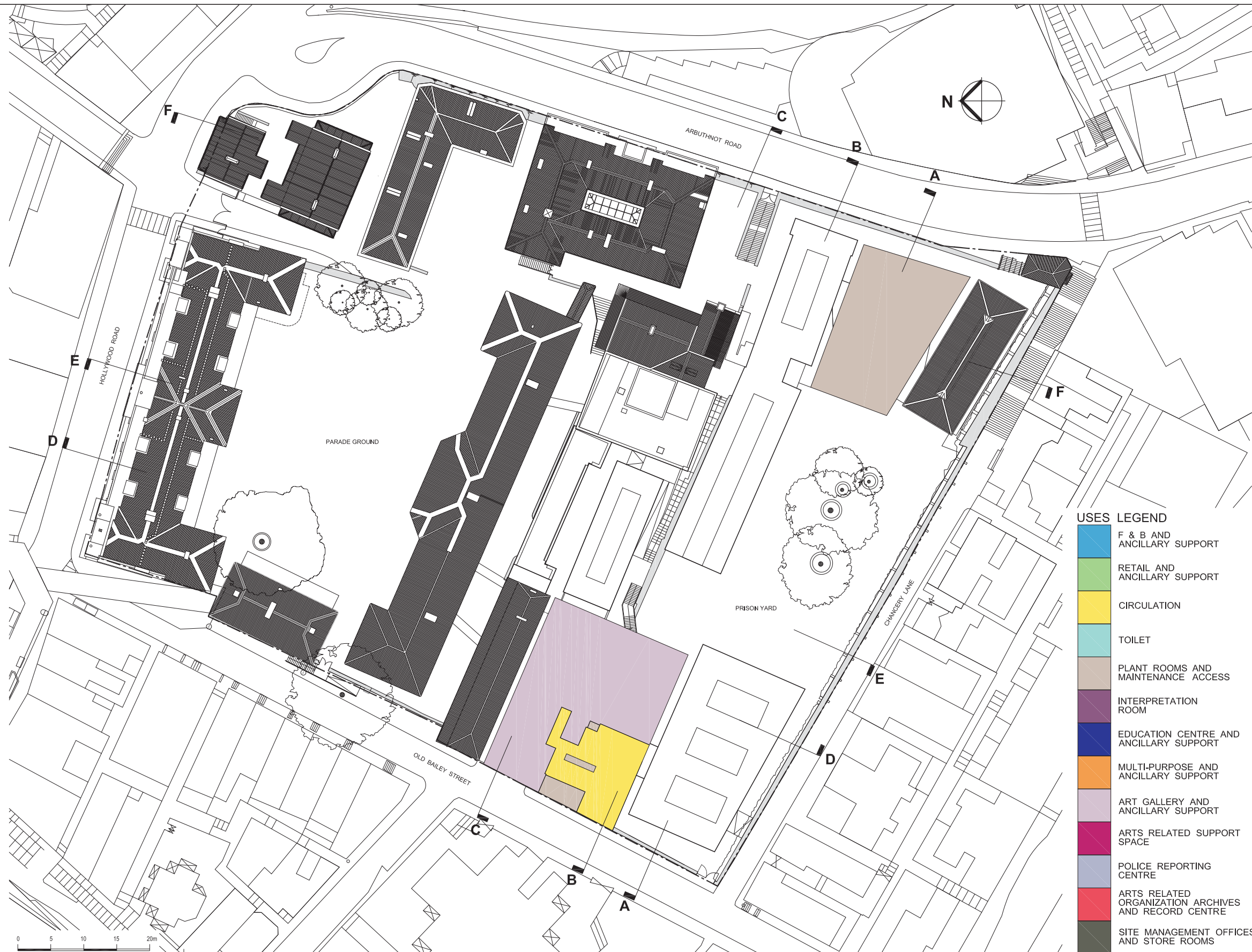
Proposed Master Layout Level 69.335
