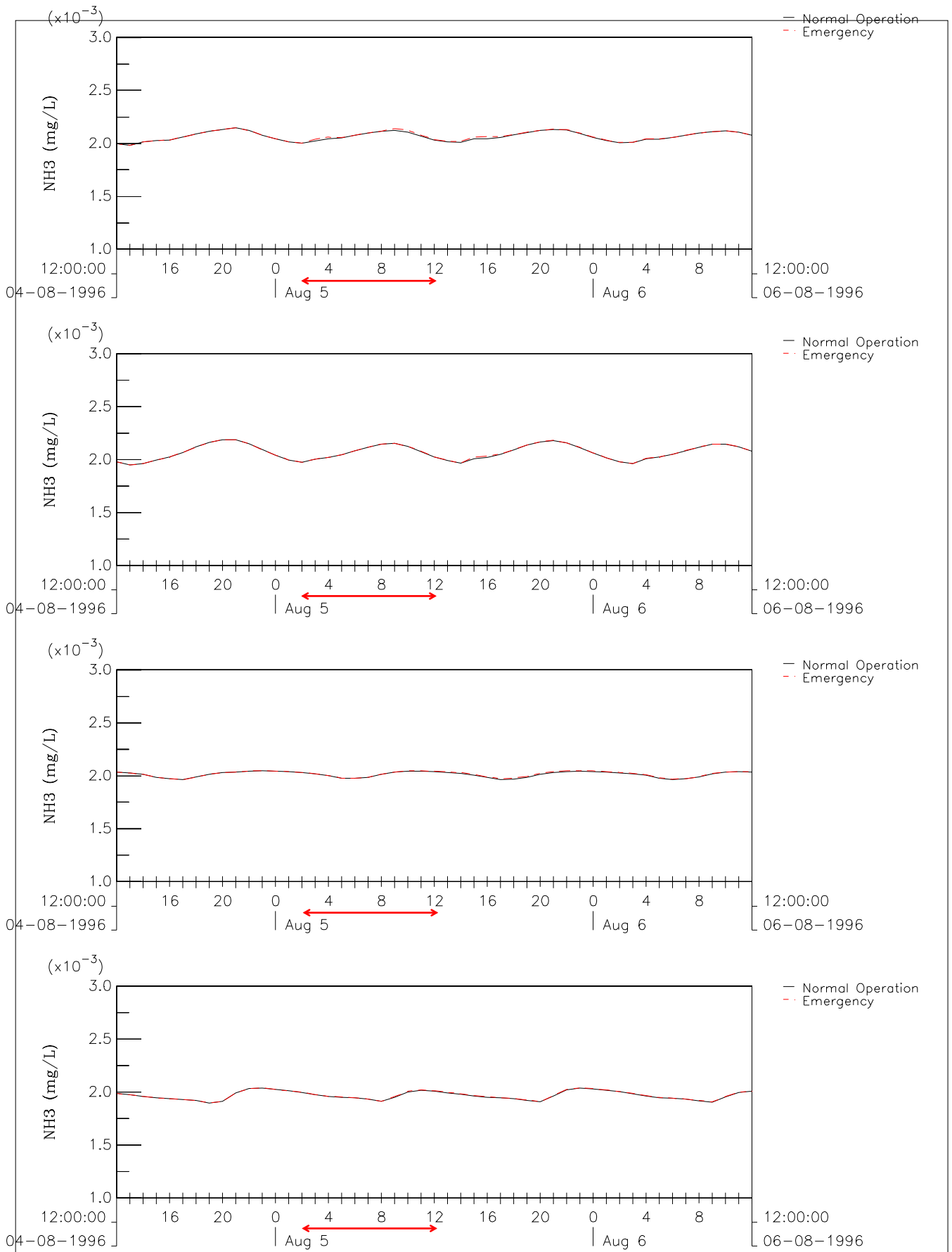
NH3 Comparison between Emergency and Normal Operation at WSR2 (TOP), WSR8 (UPPER), WSR13 (Lower) and WSR10 (Bottom). Effluent discharged at high water slack tide during the neap tide.
