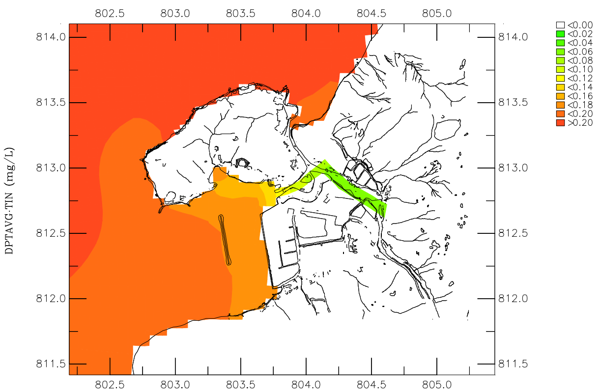
Simulated Depth Averaged TIN Normal Operation (Upper) and Maximum Concentration (Lower) occurred at 10:00 Aug 05 during Emergency Discharge Dry Season S3c High Water Slack Tide + Neap Tide DSD & ATKINS Figure 5F-15
