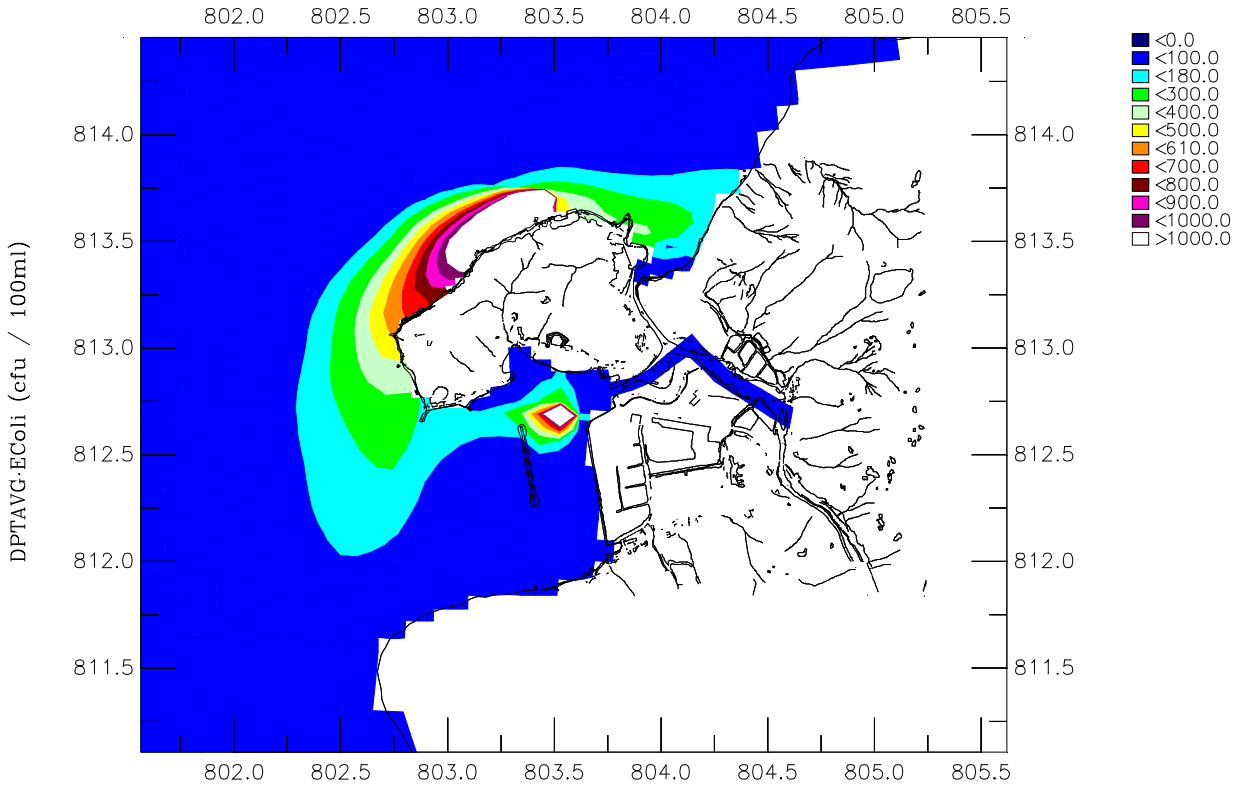
Simulated Depth Averaged EColi Normal Operation (Upper) and Maximum Concentration (Lower) occurred at 08:00 Jul 27 during Emergency Discharge.
