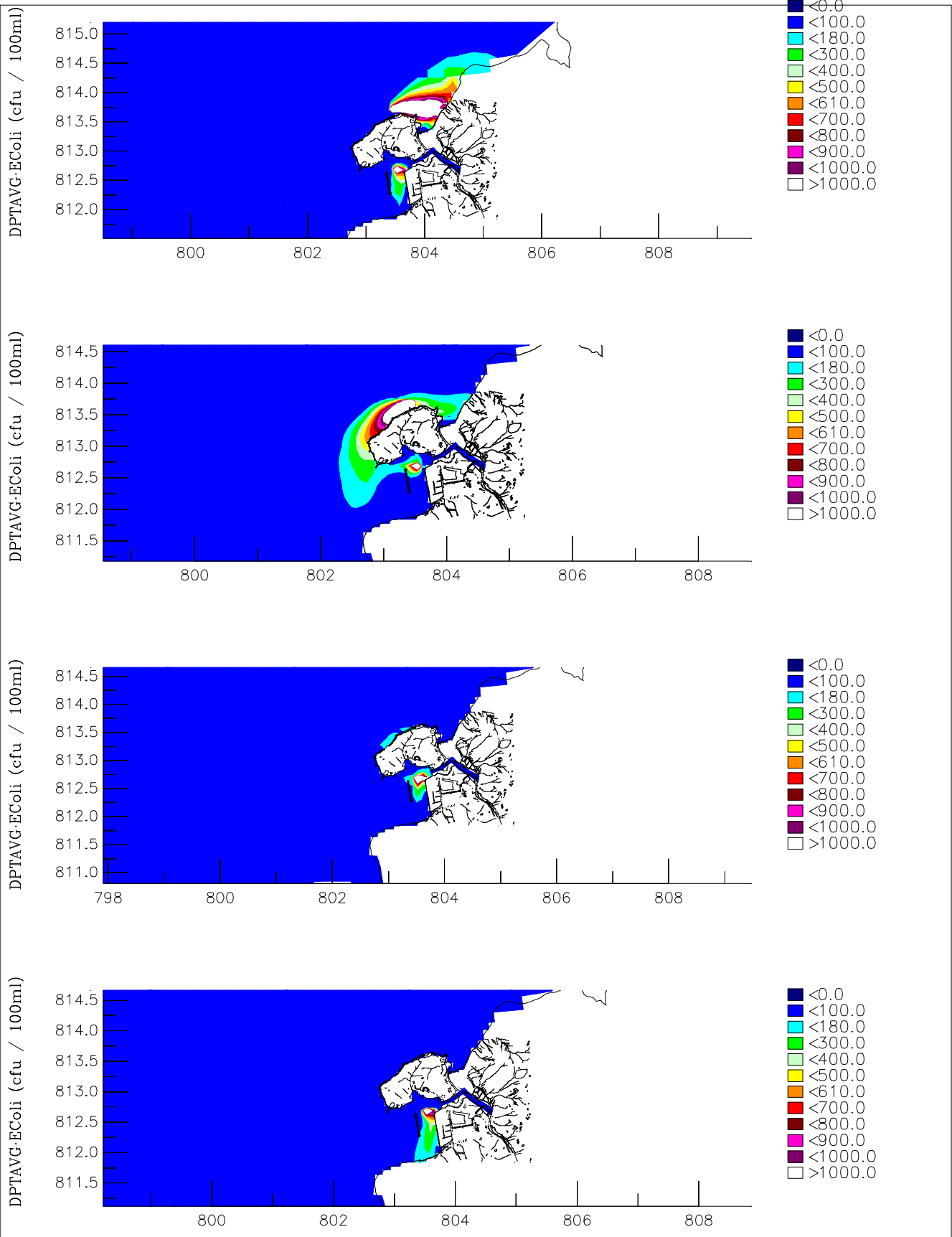
Simulated Depth Averaged EColi 1 hour, 5 hours, 9 hours, 13 hours after Emergency Discharge Wet Season S3e Flood Tide + Spring Tide DSD & ATKINS Figure 5F-22
