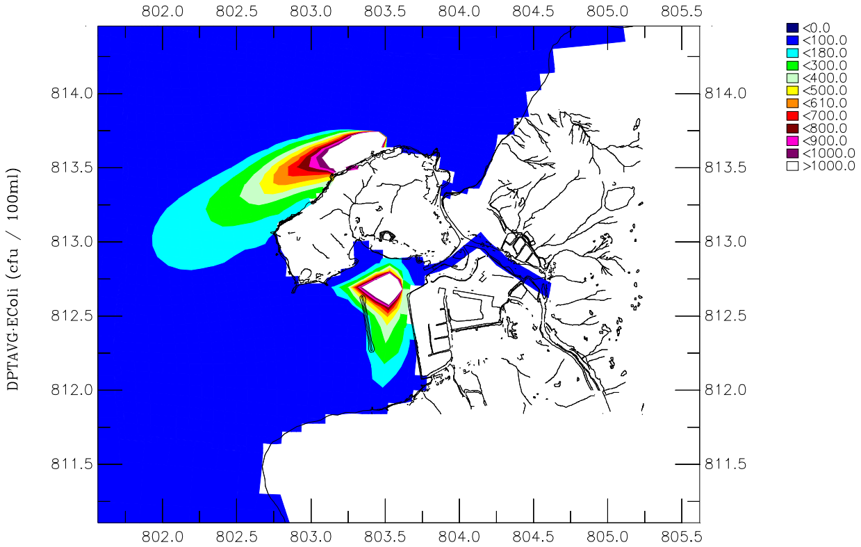
Simulated Depth Averaged EColi Normal Operation (Upper) and Maximum Concentration (Lower) occurred at 02:00 Jul 27 during Emergency Discharge. Dry Season S3b Ebb Tide + Spring Tide DSD & ATKINS Figure 5F-6
