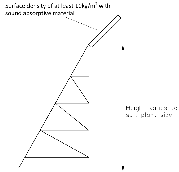
Schematic Drawing of Temporary Noise Barrier for Mobile Plant / Static Plant (~4–6m tall)
