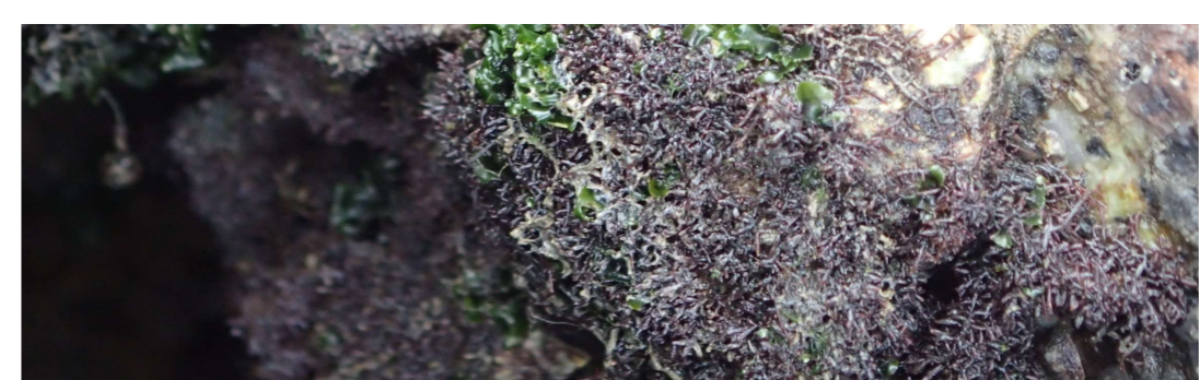
d) Algae species, Gelidium pusillum recorded at T1 and T2.
