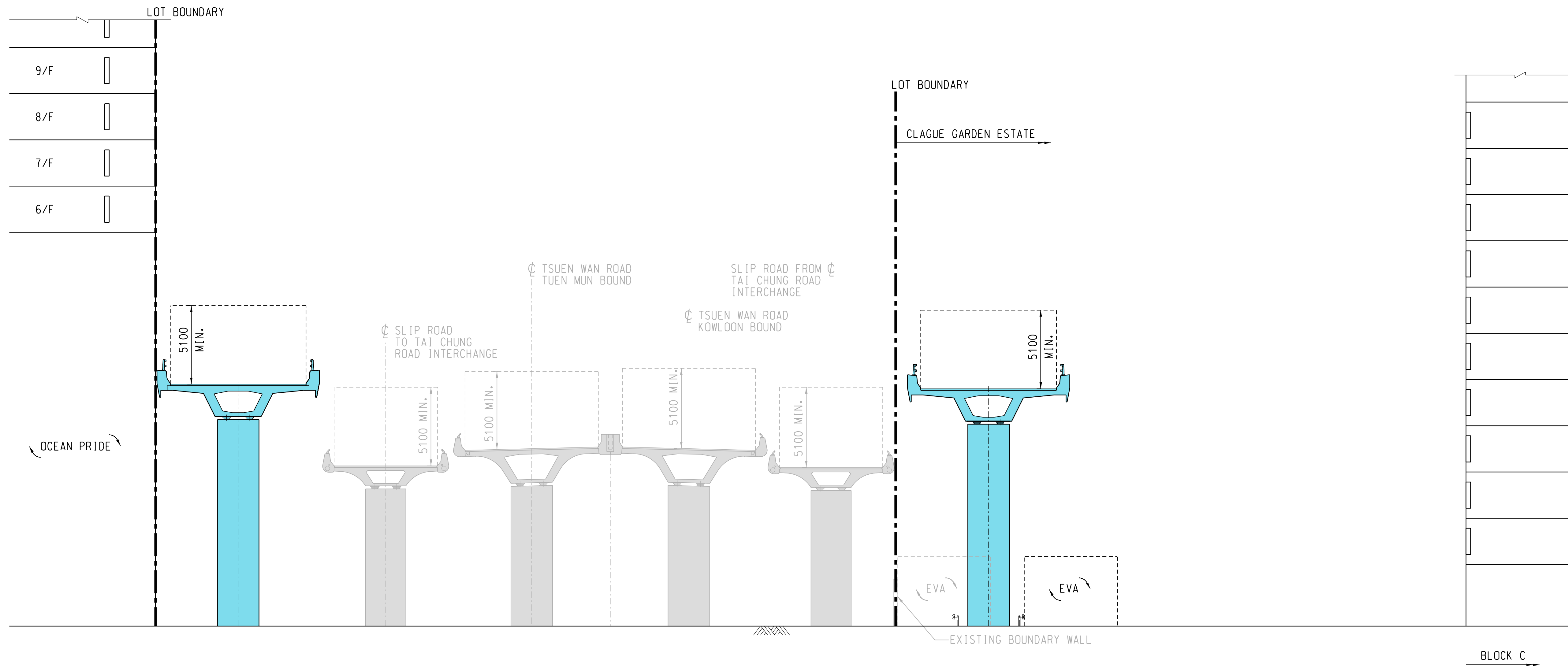
SECTION AT CLAGUE GARDEN ESTATE (SECTION A2-A2)
