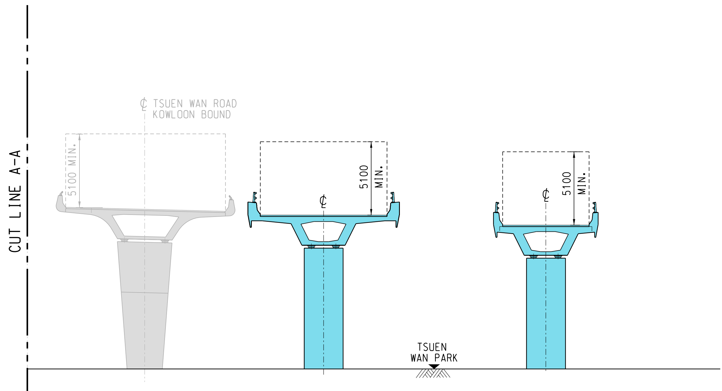
SECTION AT PAVILIA BAY (SECTION A4-A4)
