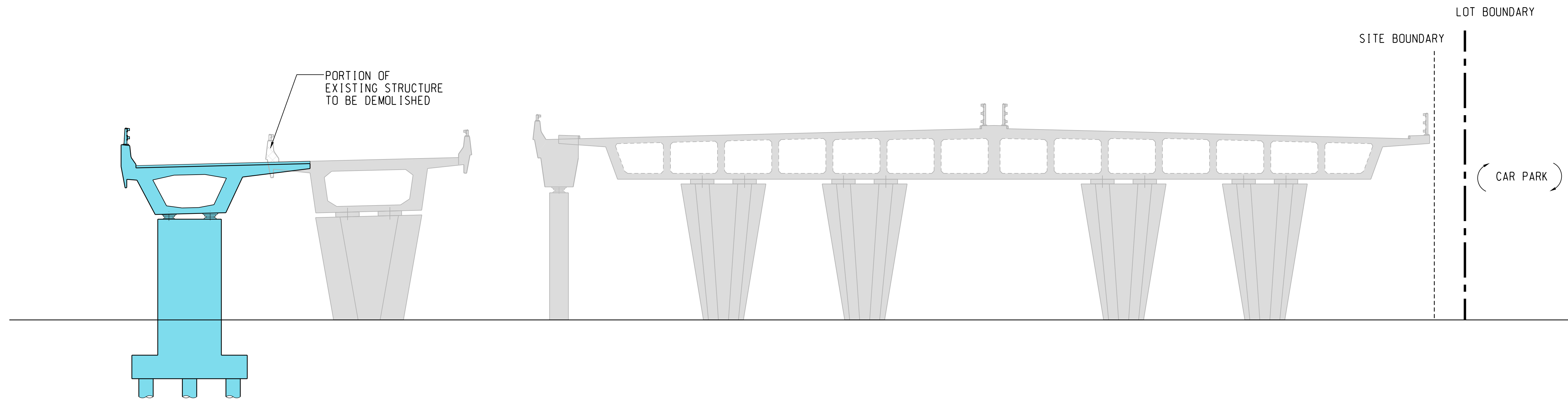
SECTION G - G
