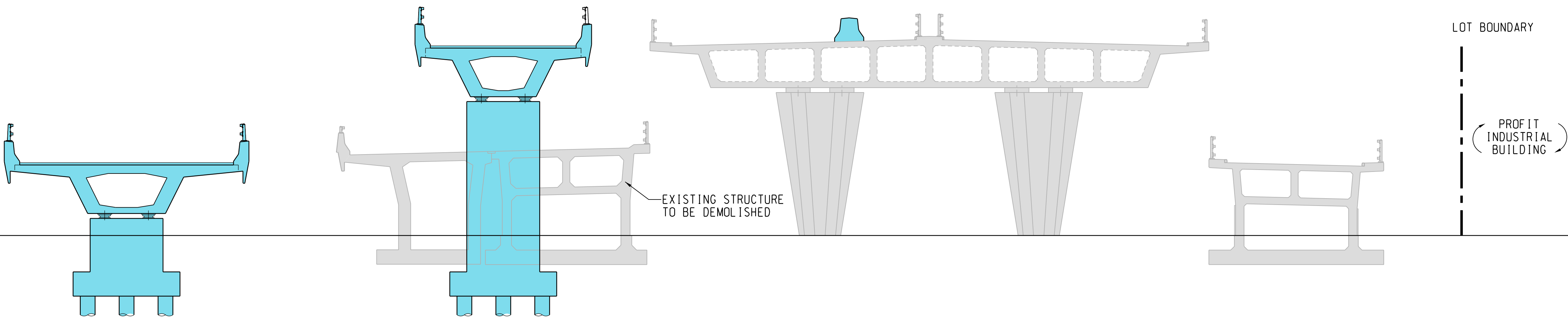
SECTION F - F
