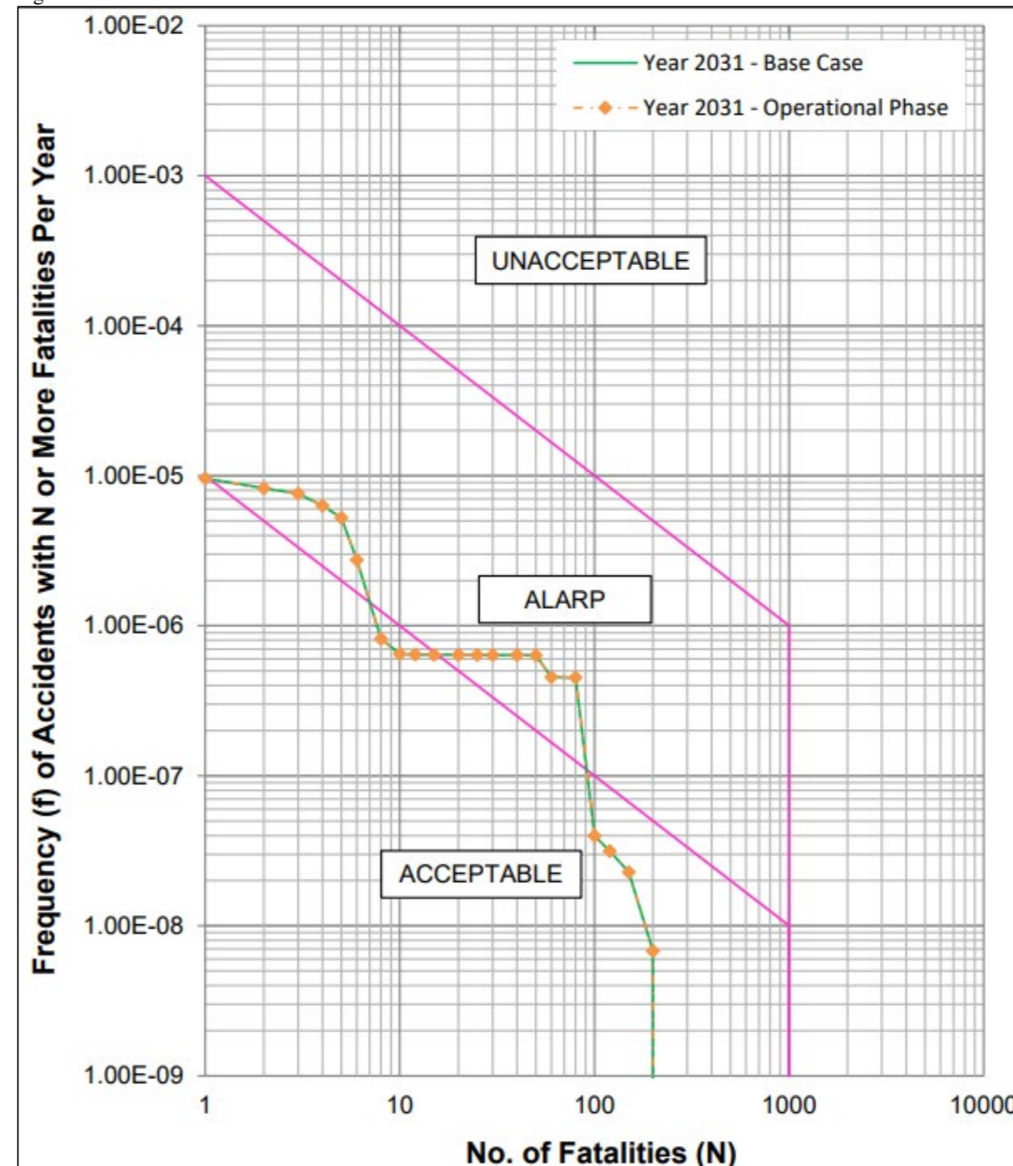
Figure LPG-2 FN Curve for TM44 LPG Store
