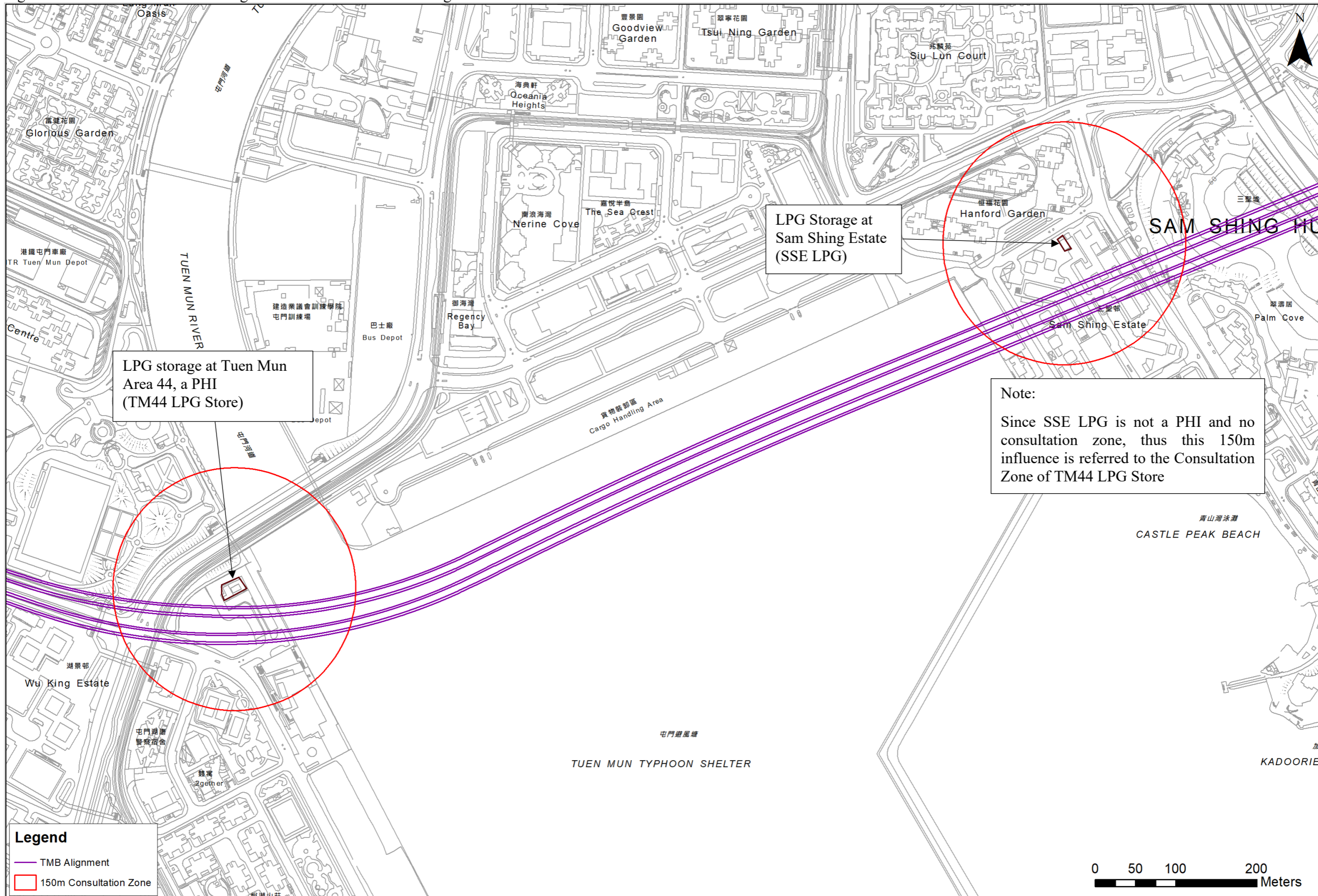
Figure LPG-1 Location of LPG Storage at TM Area 44 and Sam Shing Estate
