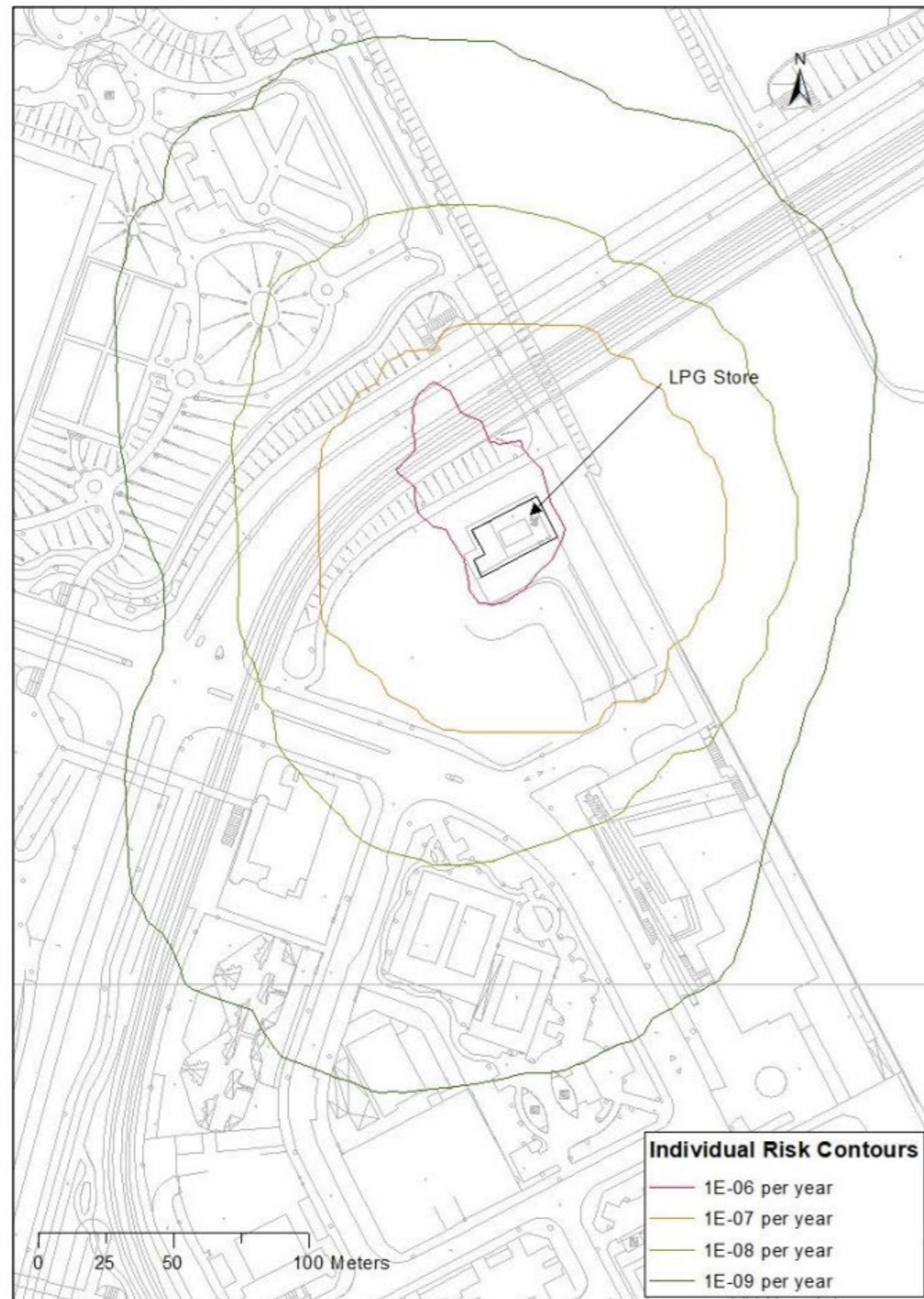
Figure LPG-3 Individual Risk Contour for TM44 LPG Store
