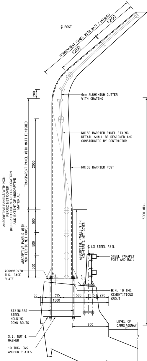
TYPICAL SECTION OF NOISE BARRIER (5m HIGH + 2.5m CANTILEVER)
