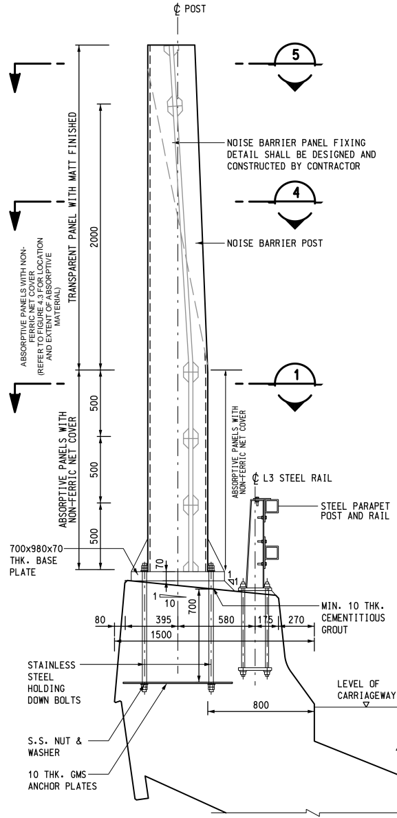
TYPICAL SECTION OF NOISE BARRIER (5m HIGH)
