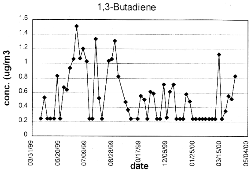
Figure 4.1a Concentrations of Selected VOCs at PolyU Station
