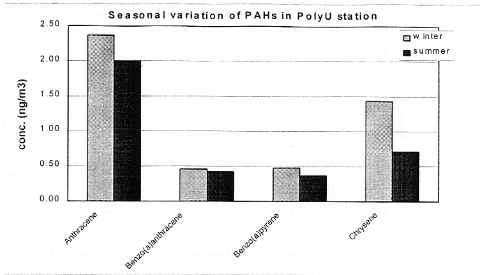
Figure 4.1m Seasonal Variation of PAHs at PolyU Station
