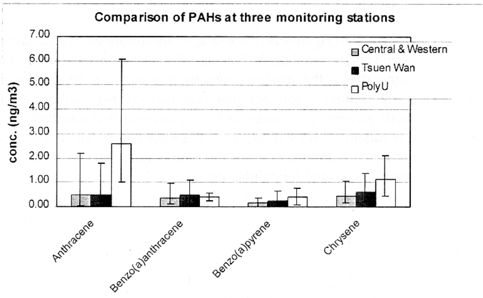
Comparison of Four Selected PAHs at the Three Monitoring Stations
