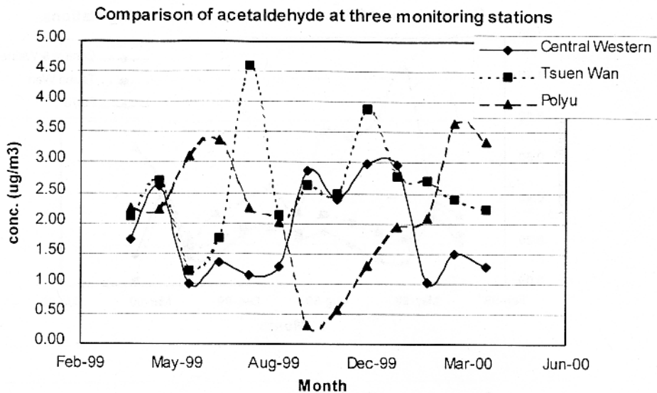
Figure 4.2e Monthly Variations of Carbonyls at the Three Monitoring Stations
