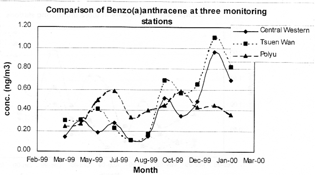
Figure 4.2f Monthly Variations of PAHs at the Three Monitoring Stations
